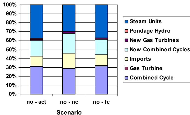
Figure 4.2 2002 Energy Displacement by Technology
