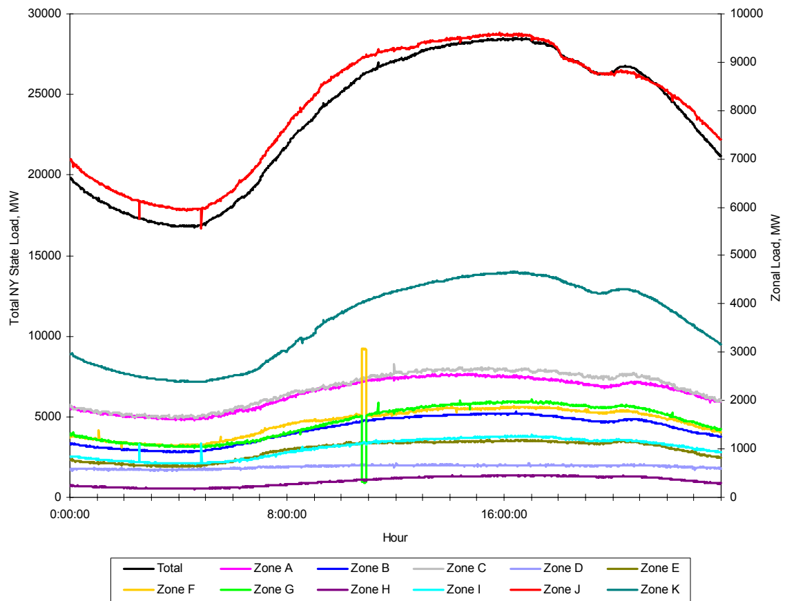
Figure 6.2 Example Load Profile from August 2003.
