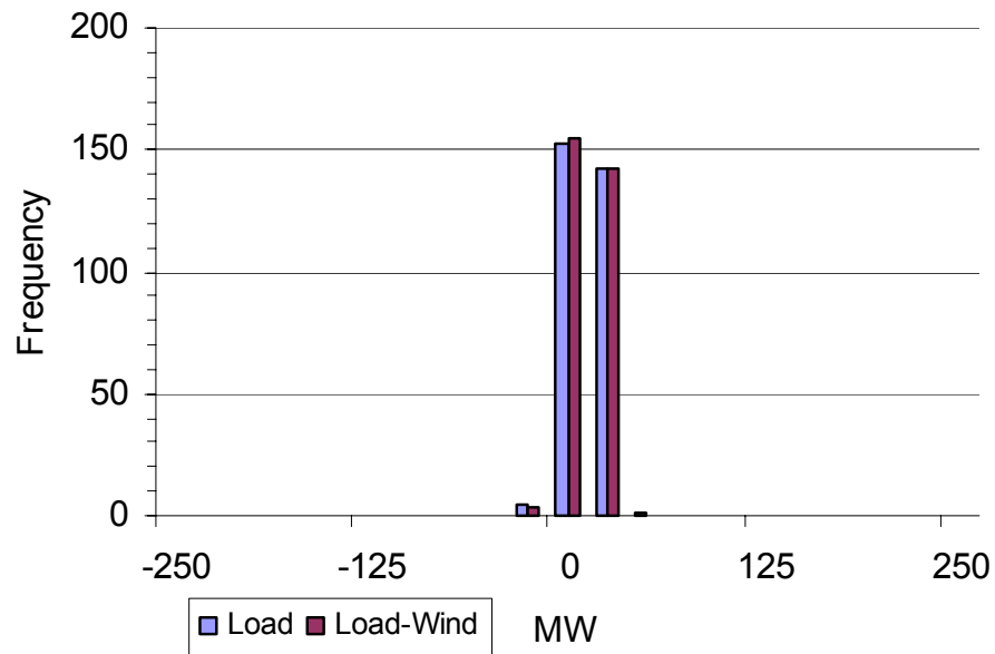
Figure 5.33 Histogram of Zone K 6-second Variance
