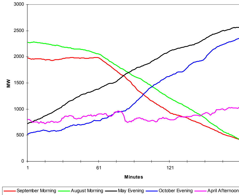
Figure 6.3 Wind Generation Study Scenarios.
