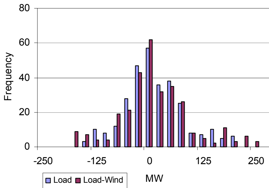
Figure 5.31 Histogram of Statewide 6-second Variance
