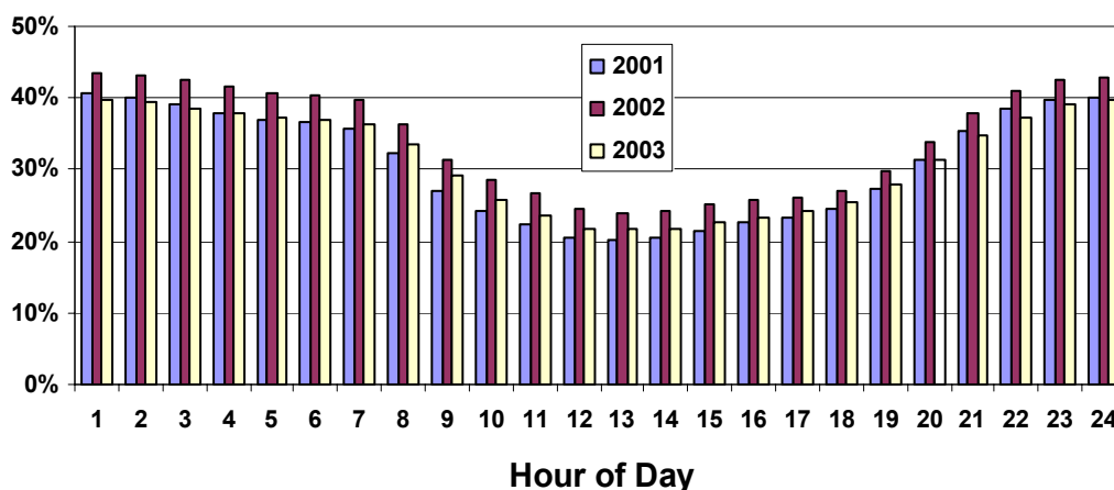
Figure 7.2 Hourly Wind Capacity Factors
