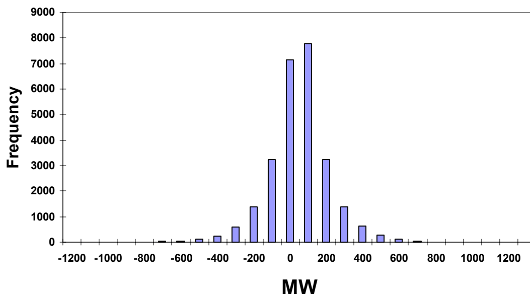
Figure 8.1. Hourly Wind Deltas, 2001 through 2003
