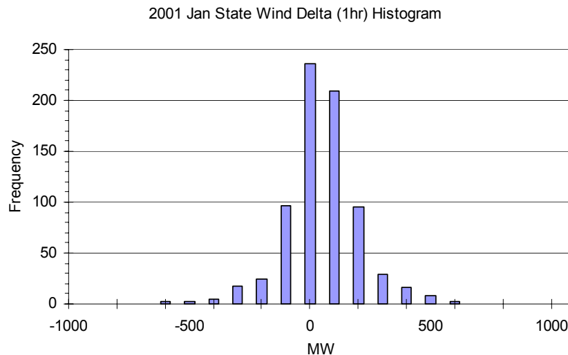
Figure 5.9 Hourly Variability of Statewide Wind Alone for January 2001
