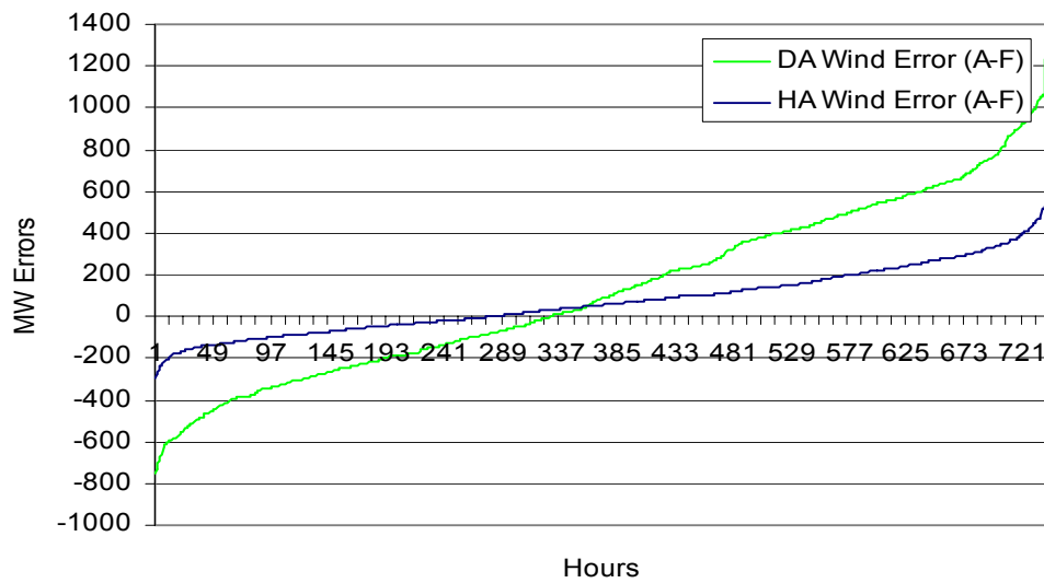
Figure 3.16 Day-Ahead and Hour-Ahead Wind Forecast Error Duration for January 2001
