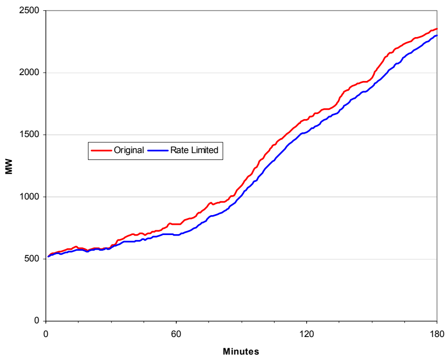
Figure 6.16 Total New York State Wind Generation with and without Active Power Control.
