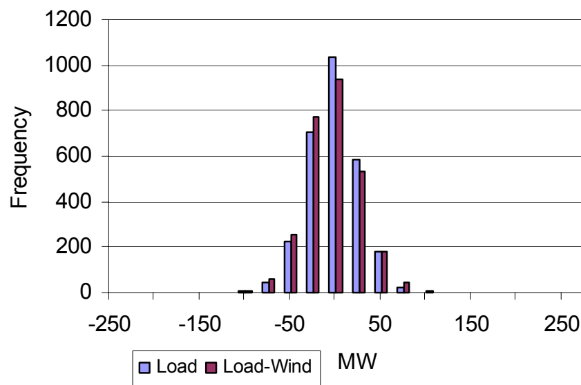
Figure 5.17 Five-minute Variability for Superzone A-E
