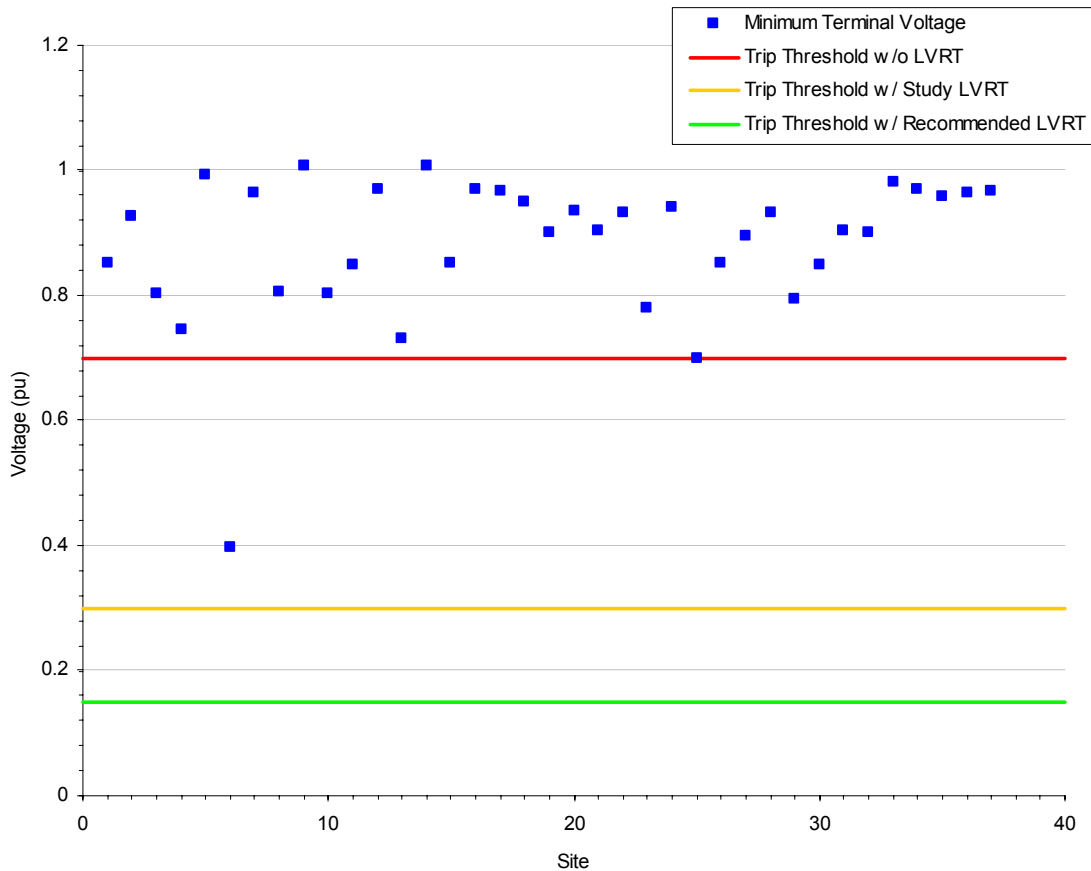
Figure 6.22 Minimum Terminal Voltages for All Wind Farms in LVRT Example.
