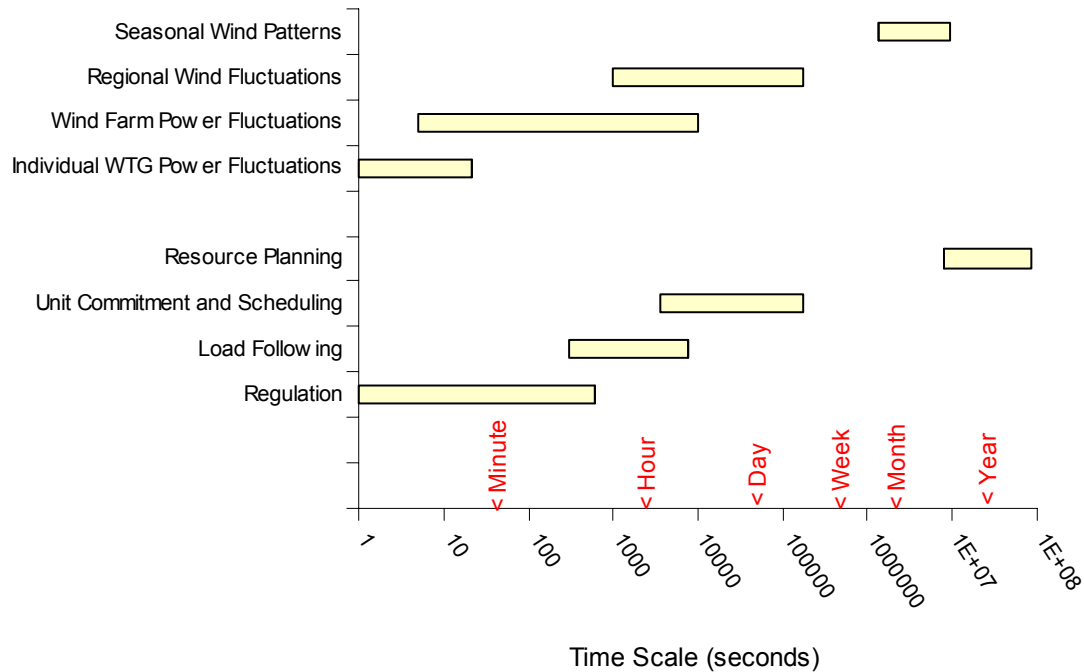
Figure 1.3 Wind Variability and Impact on System Operation Processes
