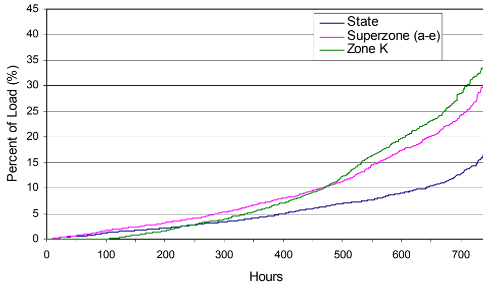
Figure 5.7 Range of Penetration based on actual wind for January 2001
