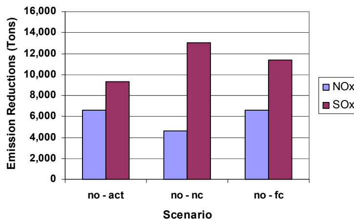
Figure 4.10 2002 Emission Reductions
