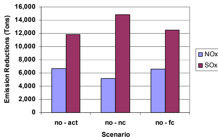
Figure 4.9 2001 Emission Reductions
