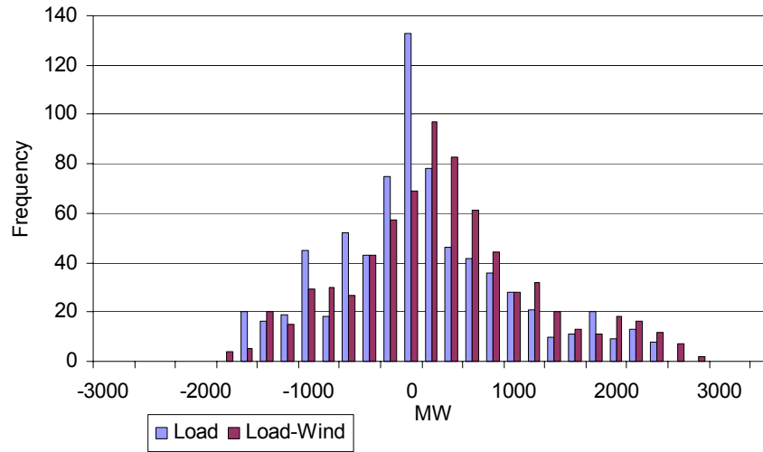
Figure 5.10 Statewide Hourly Variability for January 2001
