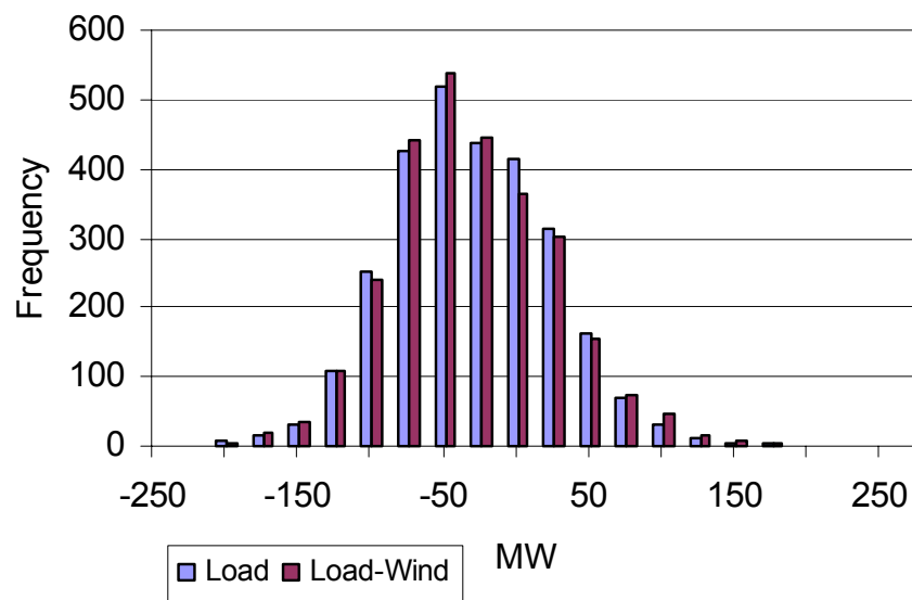
Figure 5.16 Five-minute Variability Statewide
