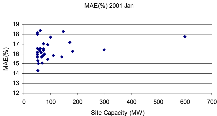
Figure 3.7 Mean Absolute Error (MAE) for Individual Wind Farms Forecasts - January 2001
