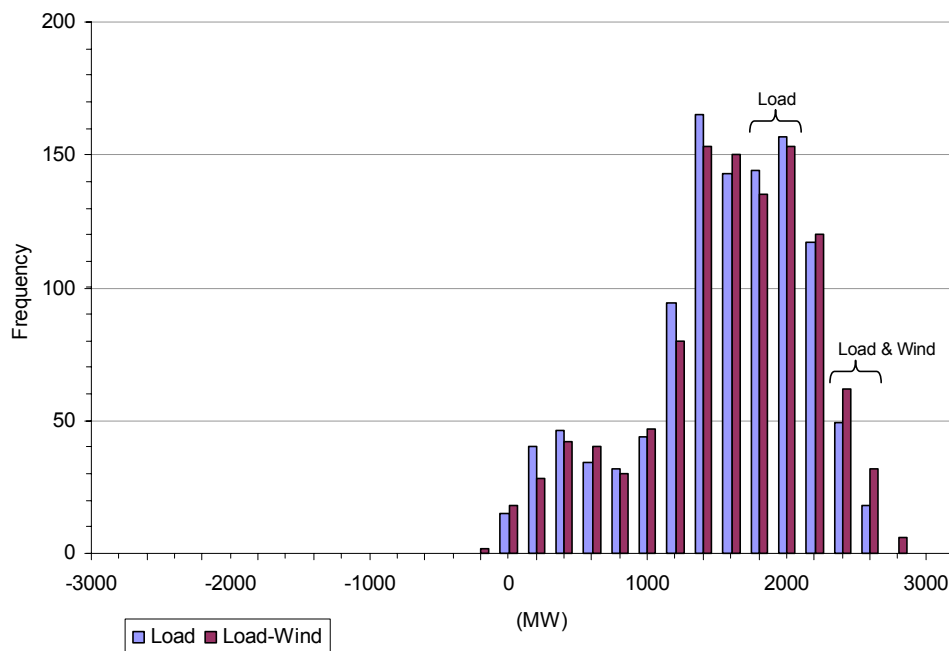
Figure 6.5 Distribution of Hourly Wind and Load Variations.
