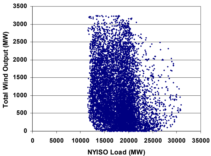
Figure 7.6 2001 Annual Load versus Wind Scatter Plot
