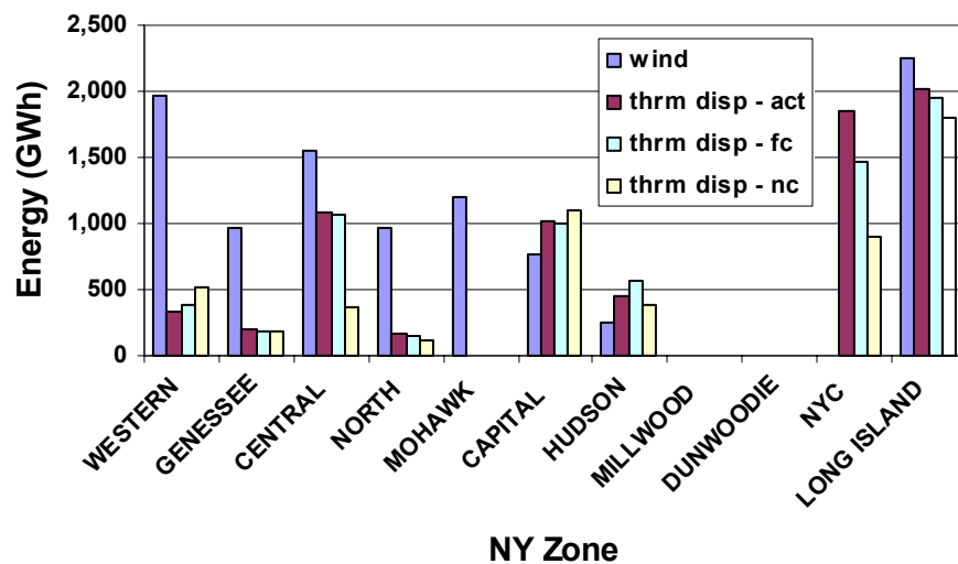
Figure 4.6 2002 Zonal Wind Generation and Displaced Thermal Generation
