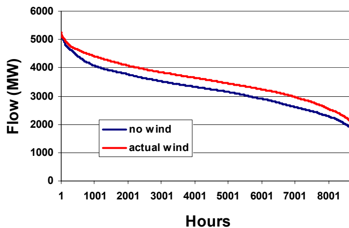
Figure 4.13 Duration Curve of Hourly Flows on Total East Interface
