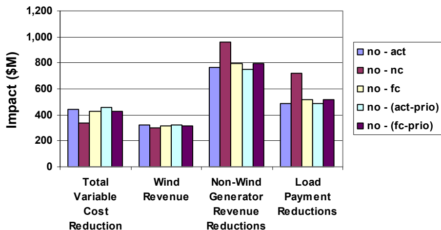
Figure 4.15 2001 Economic Impact
