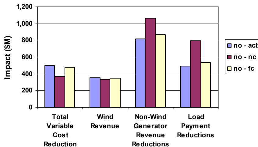
Figure 4.16 2002 Economic Impact
