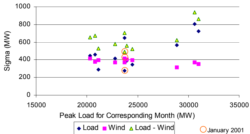
Figure 2.1 Standard Deviation of Day-Ahead Forecast Errors
