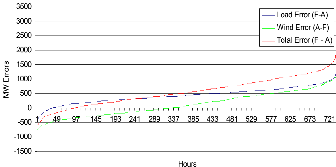
Figure 3.6 Day-Ahead Error Duration Curve for January 2001
