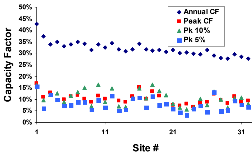
Figure 7.20 Annual and Peak Capacity Factors by Site for Year 2002 Shapes.
