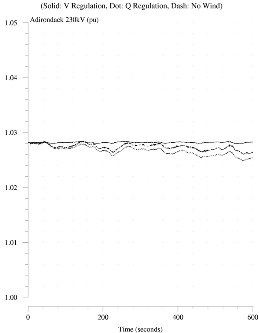
Figure 6.24 System Performance with and without Voltage Regulation.
