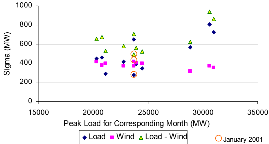
Figure 3.8 Standard Deviation of Day Ahead Forecast Errors
