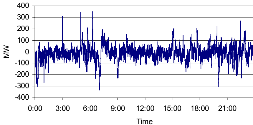
Figure 5.23 NYISO ACE for January 8, 2003
