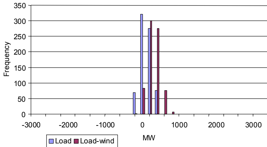
Figure 5.12 Zone K Hourly Variability for January 2001
