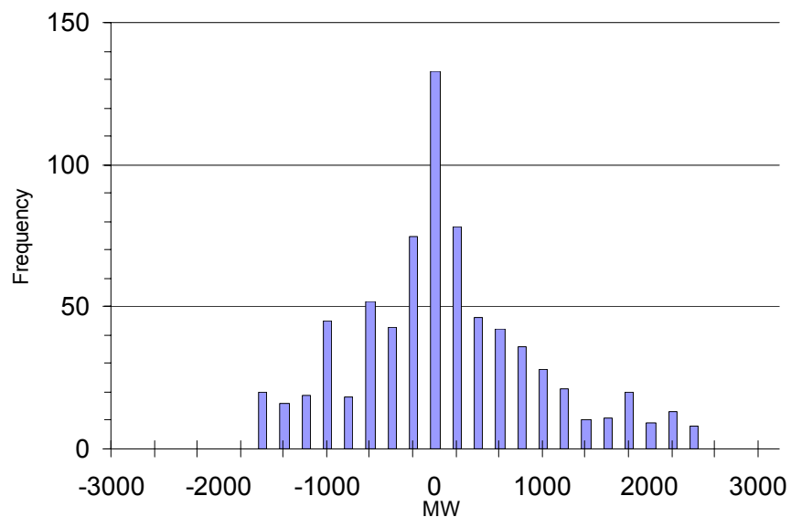
Figure 5.5 January 2001 Hourly Load Change
