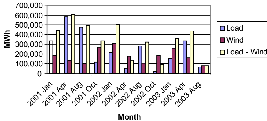
Figure 3.11 Positive Energy Error for Day-Ahead Forecasts
