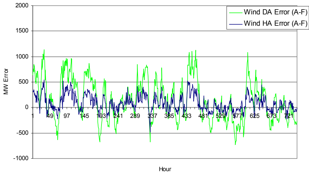
2002 NYISO Wind Forecast Error (F-A) October
