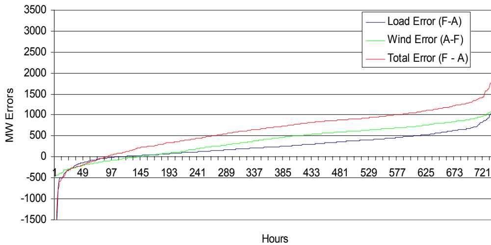
2002 January Day Ahead Forecast Errors
