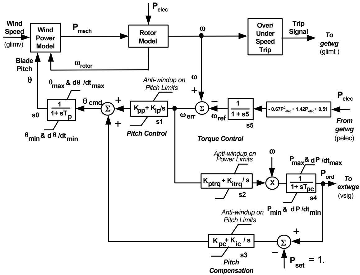
Figure D-3. Wind Turbine Model (wndtge) Block Diagram.
