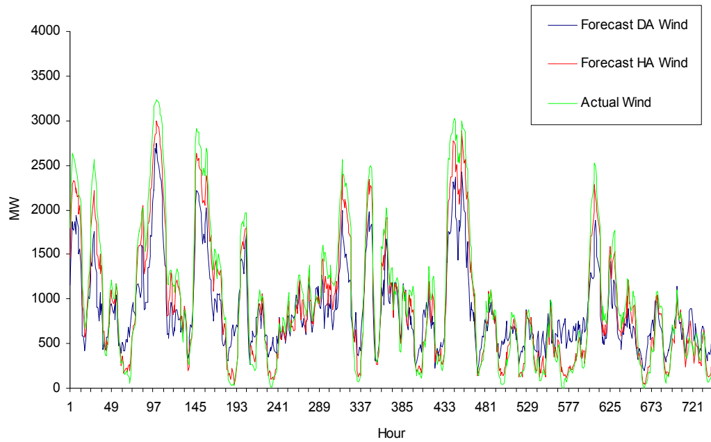
2002 October Wind
