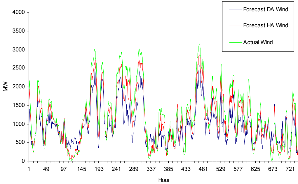
2003 January Wind
