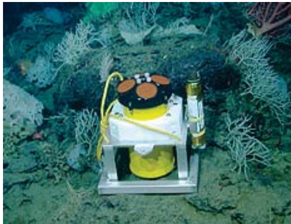
Figure 3.5: Bottom-Mounted ADCP 21
