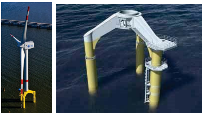
Figure 3.17: Tripile Foundation 40,41
