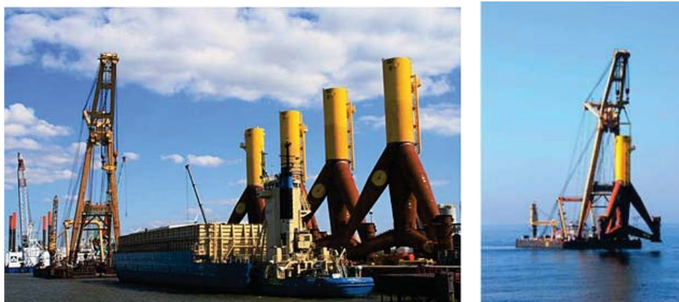
Figure 3.16: Tripod Foundation 38,39
