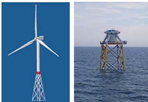
Figure 3.15: Jacket Foundation 36,37
