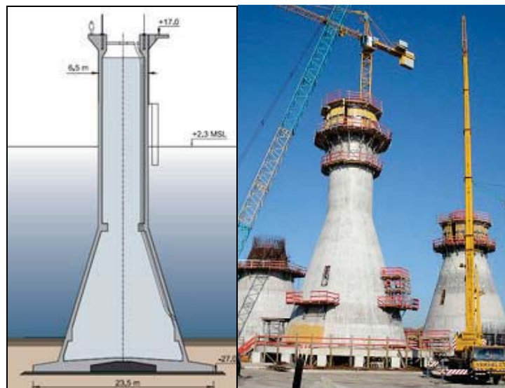
Figure 3.14: Gravity Base Foundation 35
