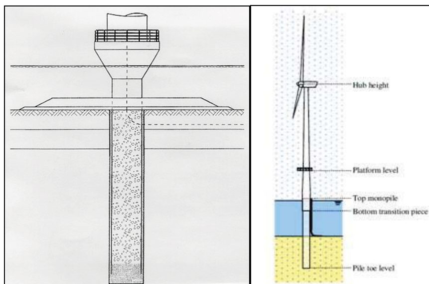
Figure 3.13: Monopile Foundation 33,34
