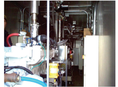
Engine modules housed inside shipping container
