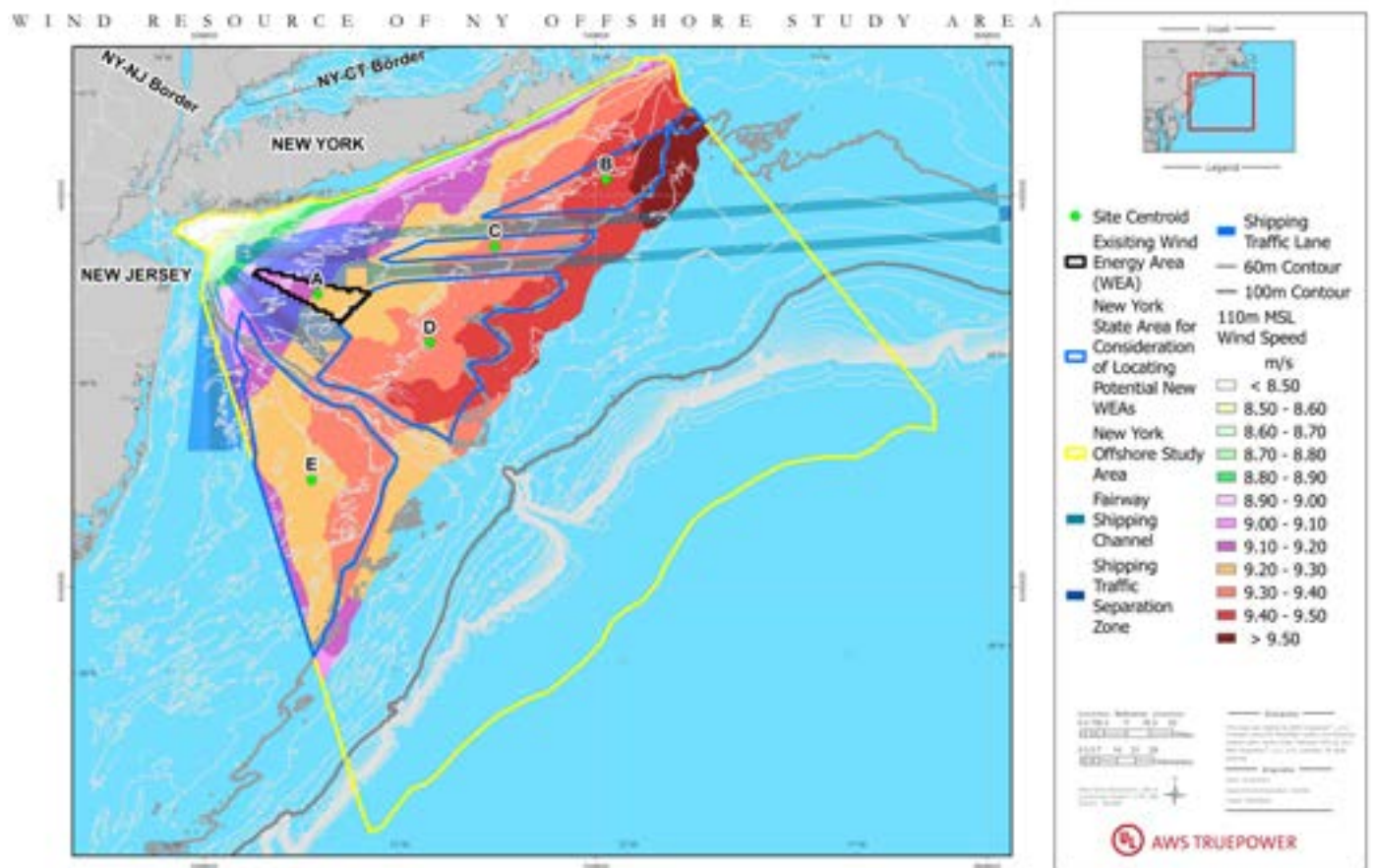
Figure 28. Wind Resource Offshore New York.
