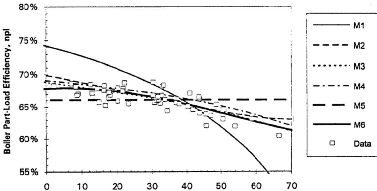
FIGURE 7.4 MODEL PREDICTIONS AND MEASURED DATA OF PART-LOAD EFFICIENCY FOR WATER BOILER IN CONSTANT TEMPERATURE MODE
