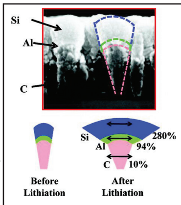
Photo of nanoscoops showing their expansion as lithium ions penetrate the silicon.
