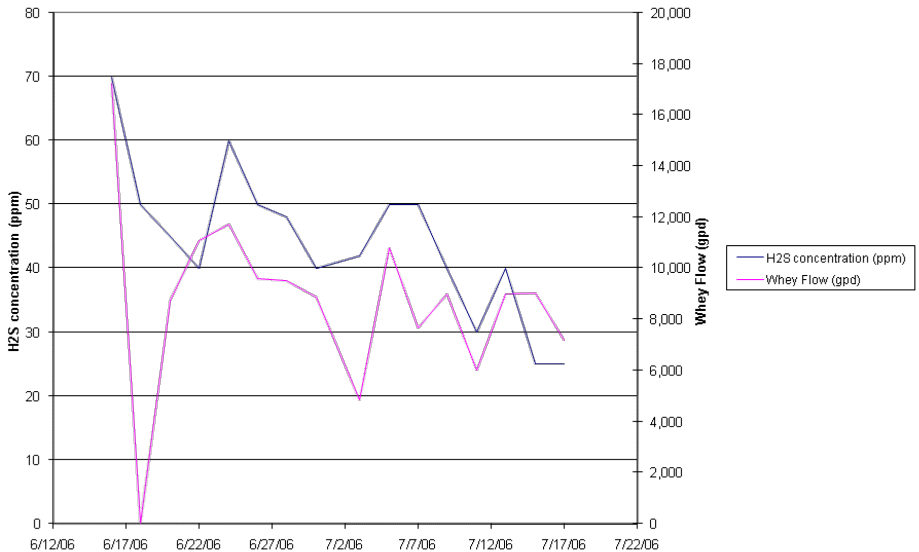
Figure 2-4: Whey Flow vs. H2S concentration
