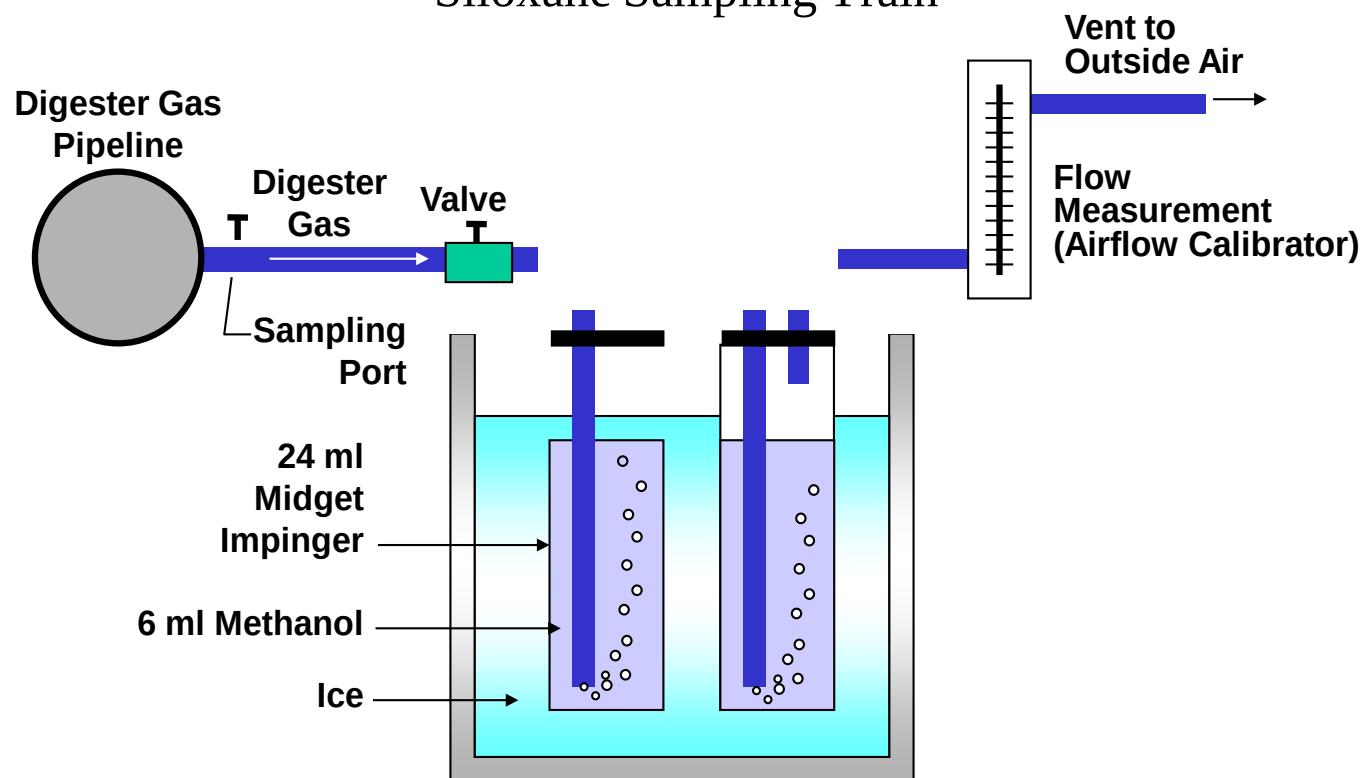
Figure 2-2 Siloxane Sampling Train
