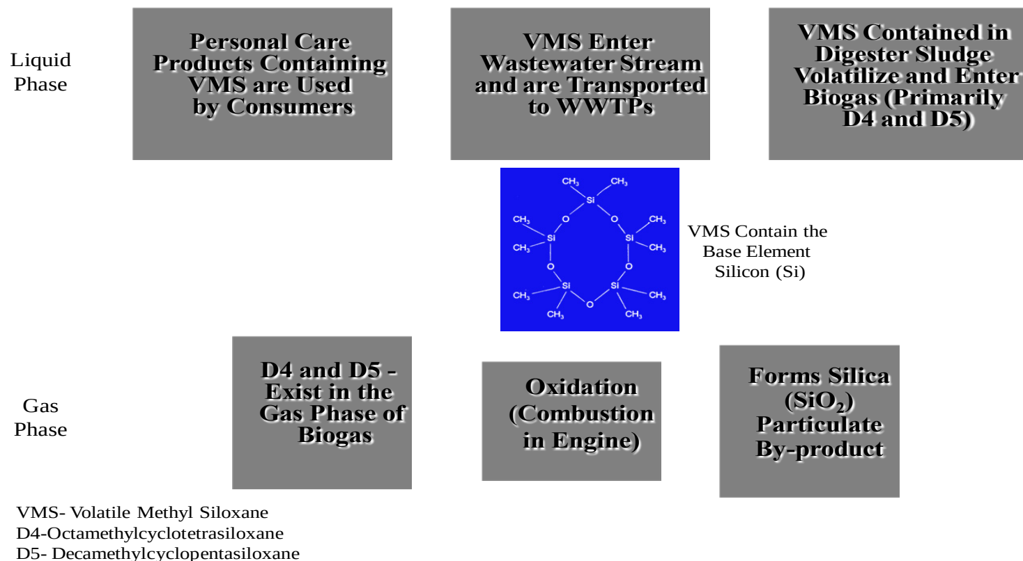
Figure 2-1 Fate of Siloxanes in WWTPs
