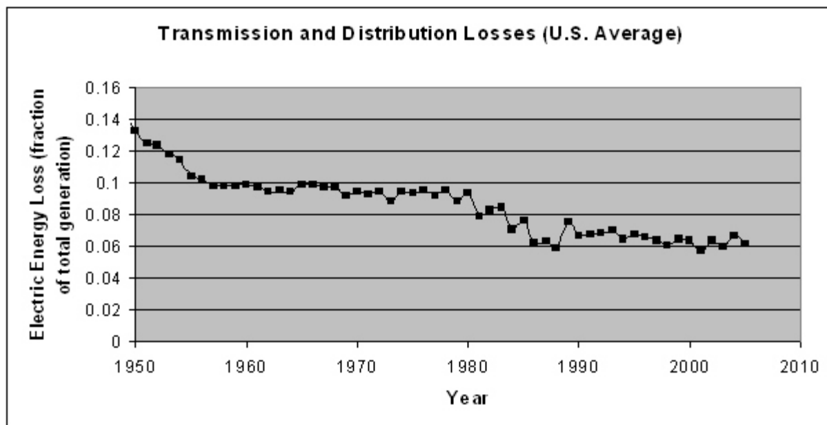
Figure 4: T&D Electric Power Losses (U.S. Average)
