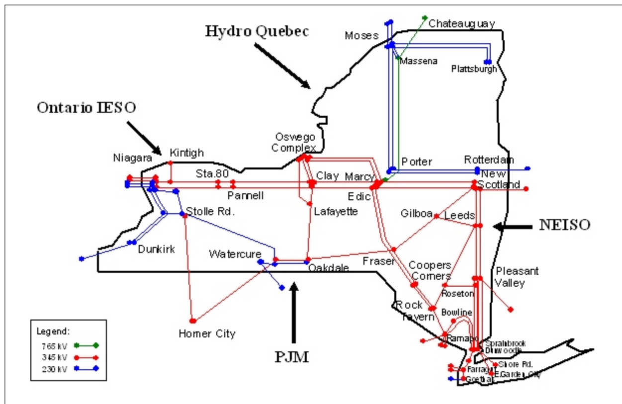
Figure 6: NYISO Regional Interconnections (NYISO)
