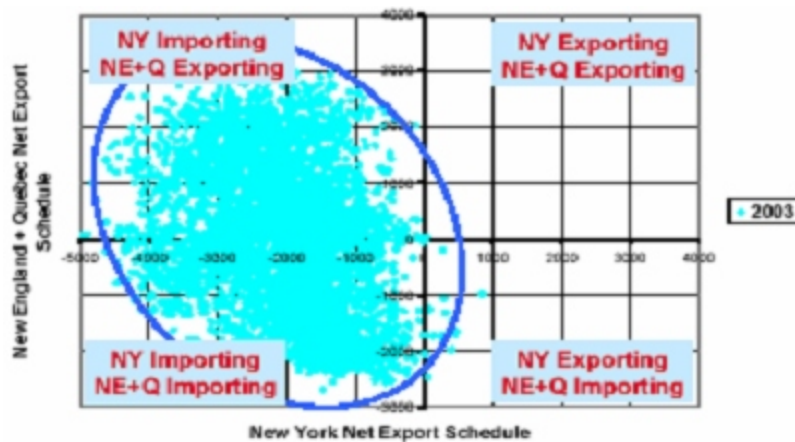
Figure 8: Wholesale Electric Power Flow (in MW) for May to October 2003
