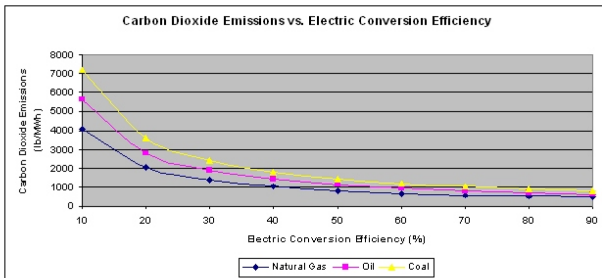
Figure 9: Comparative CO 2 Emissions Performance of Power Plants with Different Fuels
