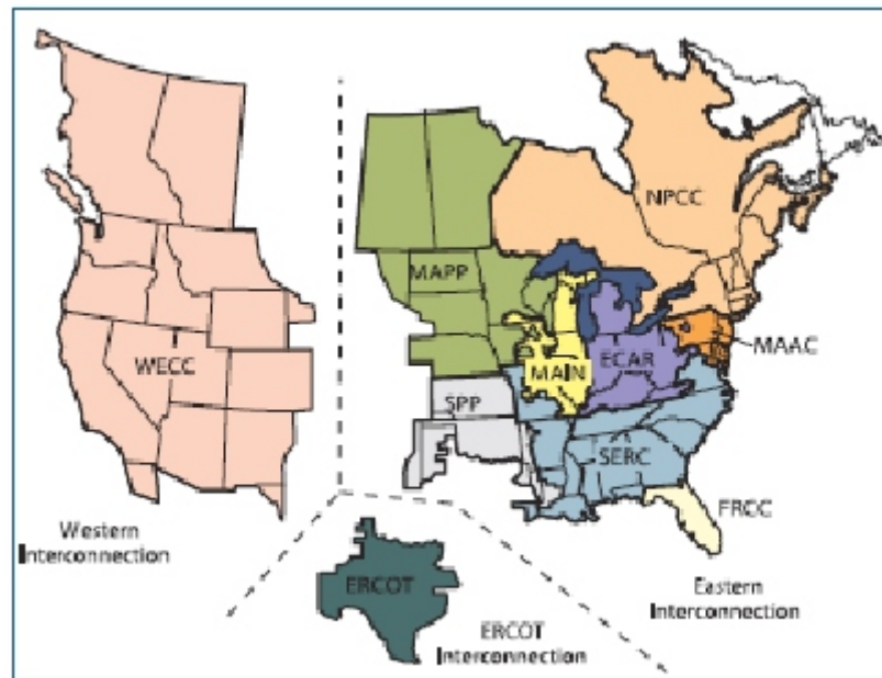
Figure 5: National/Regional Electric Power Delivery System (Source: U.S.-Canada Power System Outage Task Force: August 14 th , 2003 Blackout Study)
