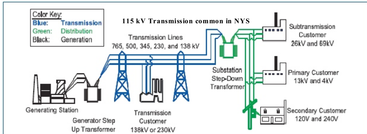
Figure 1: Simplified Transmission and Distribution System Schematic (Source: U.S.-Canada Power System Outage Task Force: August 14 th , 2003 Blackout Study)
