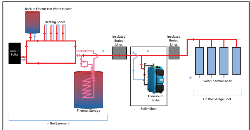
A simplified schematic of the heating system at the Hidley Farm. The heating zones take hot water to radiators throughout the farmhouse, and a radiant floor in the renovated kitchen.
