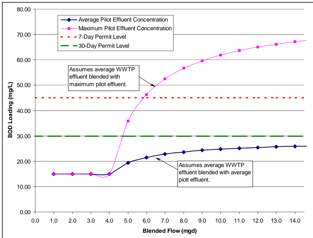
Figure 6.2. Projected BOD Concentration in Blended Effluent
