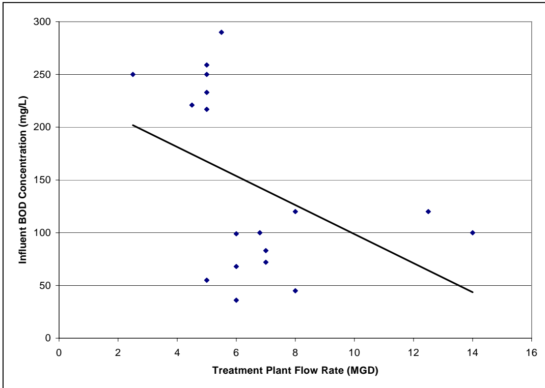
Figure 5.2. Influent BOD Concentrations as a Function of Flow Rate
