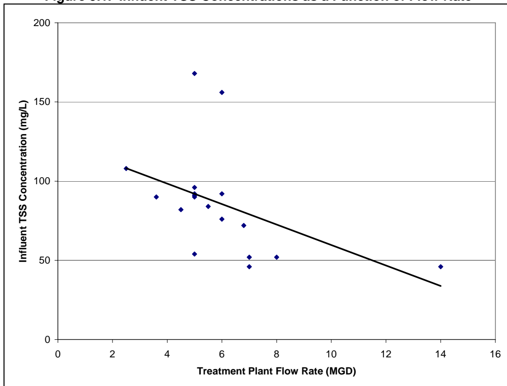
Figure 5.1. Influent TSS Concentrations as a Function of Flow Rate
