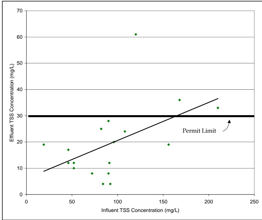
FIGURE 5.4. Effluent TSS Concentration as a Function of Influent TSS Concentration
