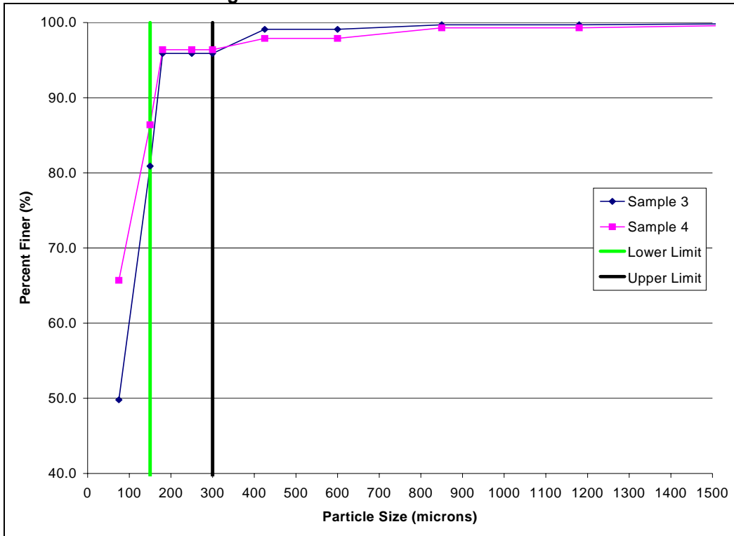
Figure 5.3. Particle Size Distribution
