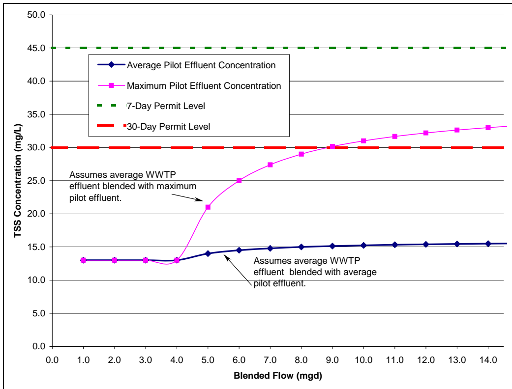
Figure 6.1. Projected TSS Concentration in Blended Effluent
