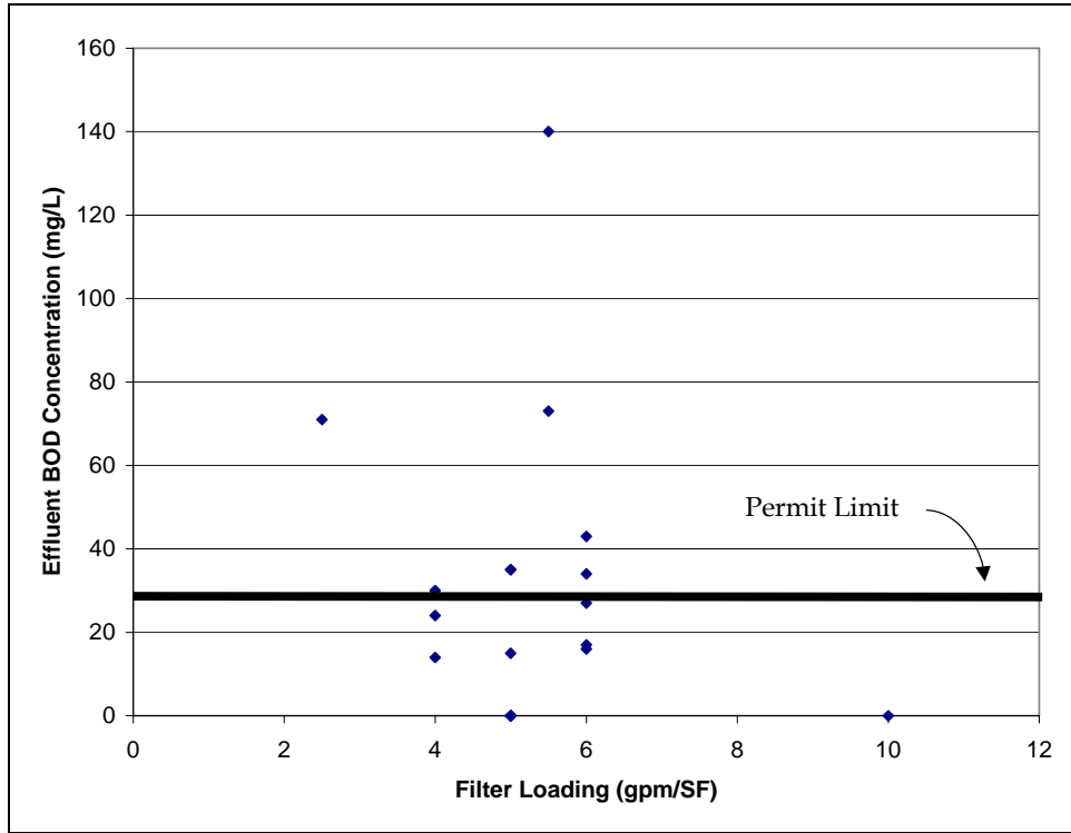
Figure 5.6. Effect of Filter Loading Rate on Effluent BOD Concentration
