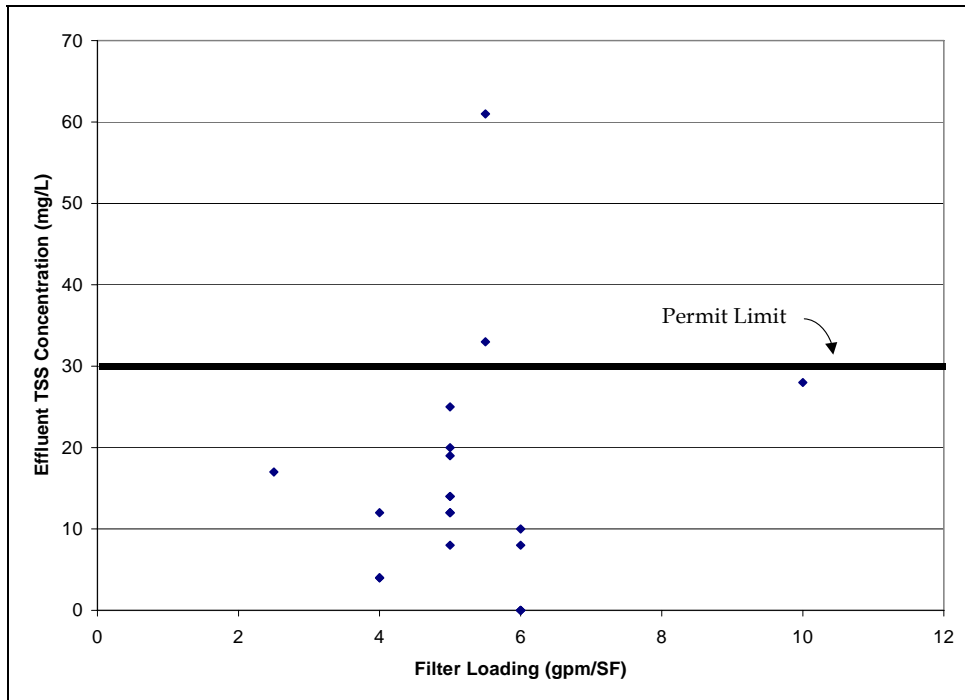
Figure 5.5. Effect of Filter Loading Rate on Effluent TSS Concentration
