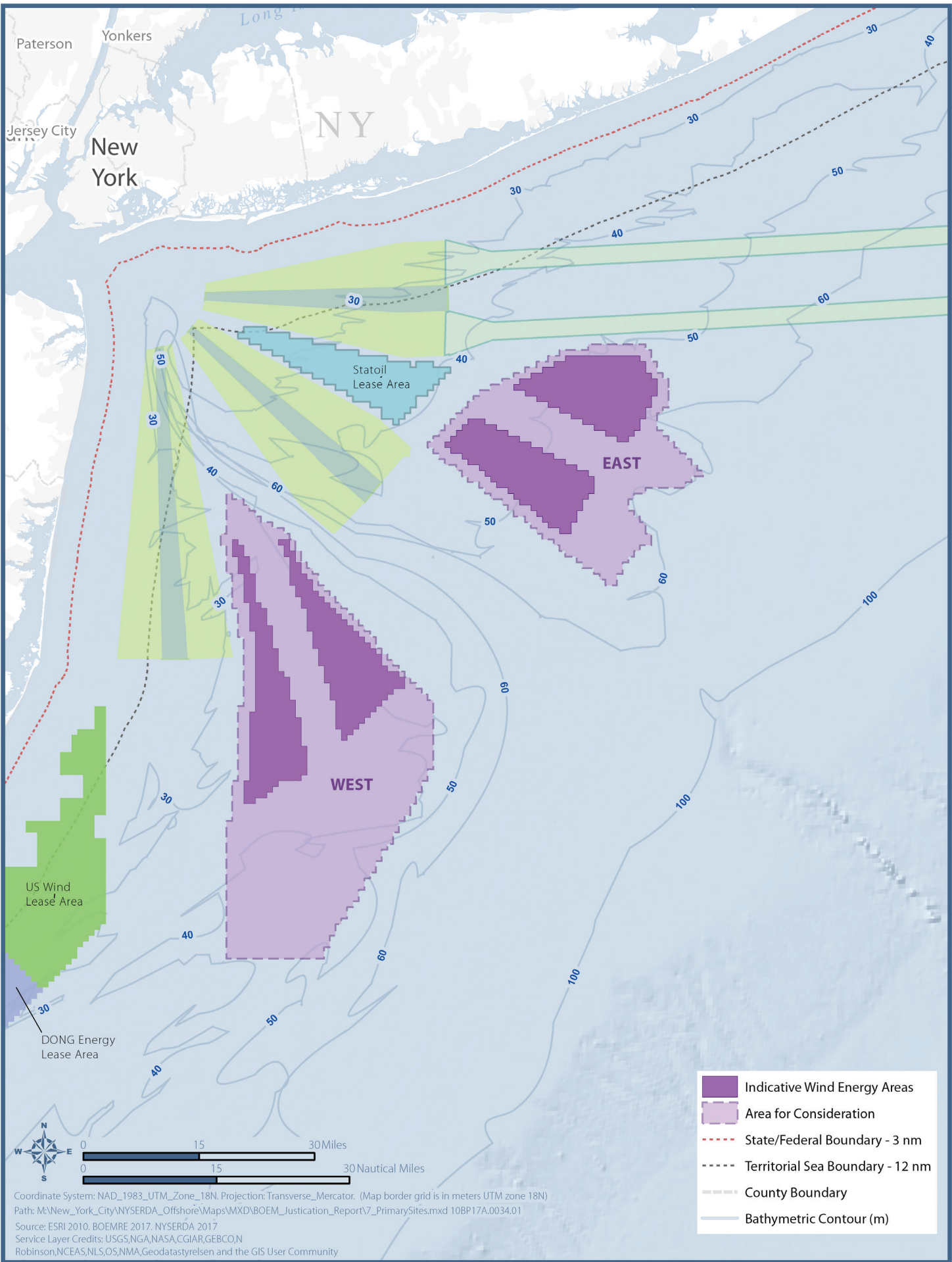
Indicative Wind Energy Areas – Configuration A.
