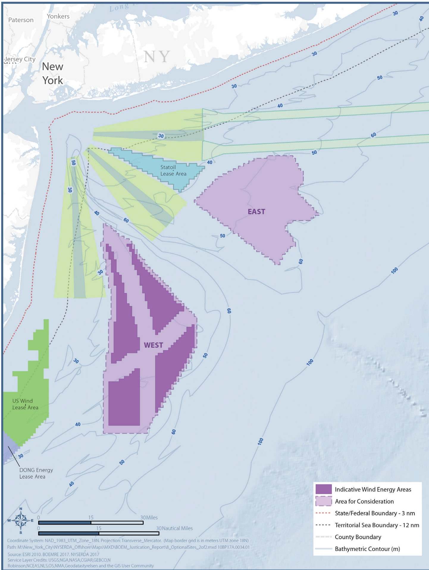
Indicative Wind Energy Areas – Configuration C.
