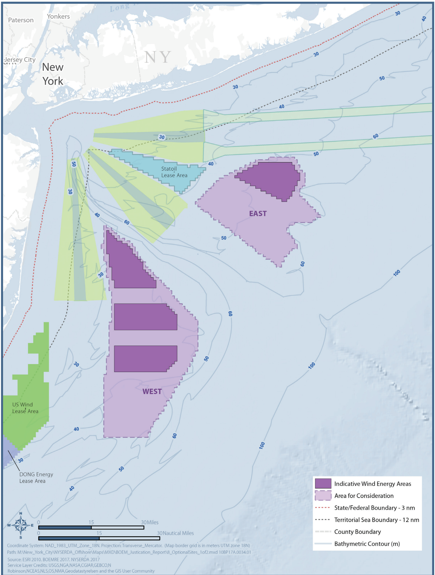
Indicative Wind Energy Areas – Configuration B.
